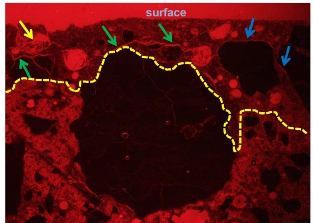
Microphotograph of the surface of concrete affected by fire, showing the depth of thermally-altered paste (yellow line) and associated cracks within the paste (arrows).
